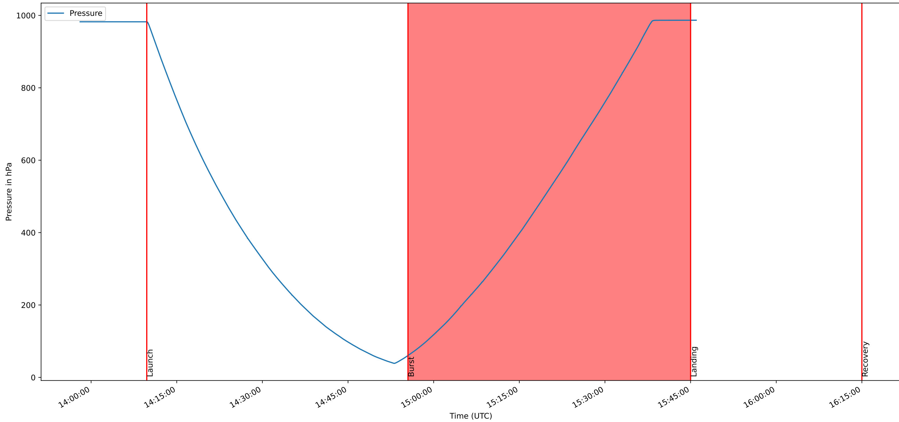
LX-187-B Pressure Plot
