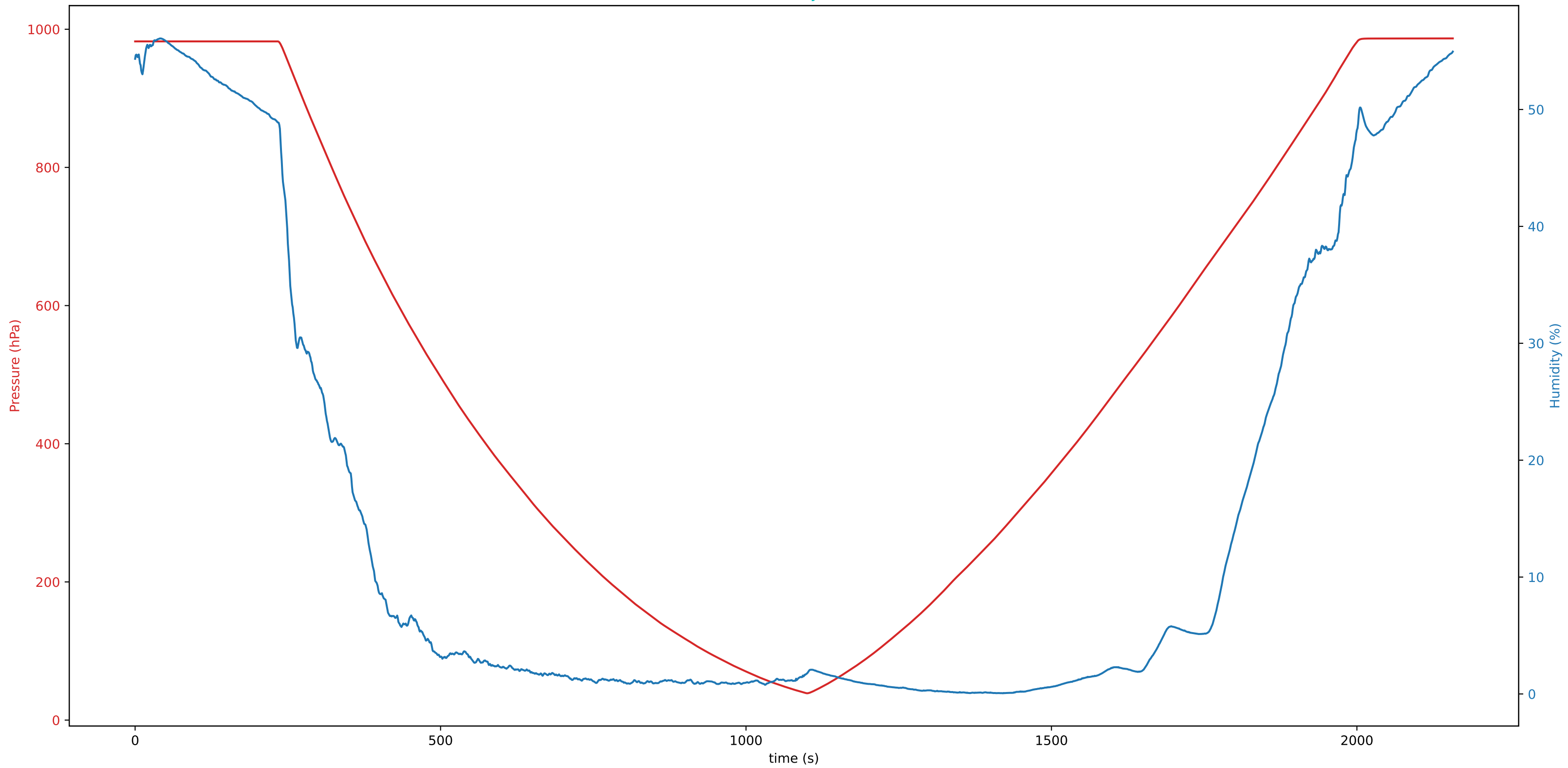
LX-187-B Humidity vs Pressure
