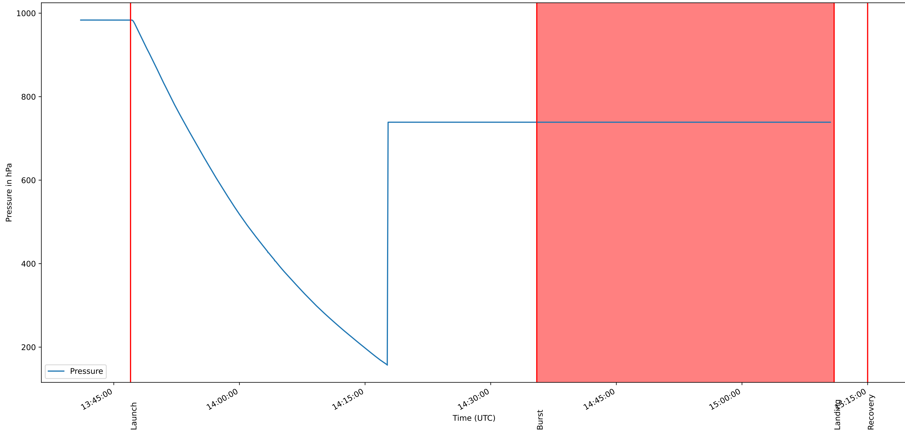
LX-187-A Pressure Plot
