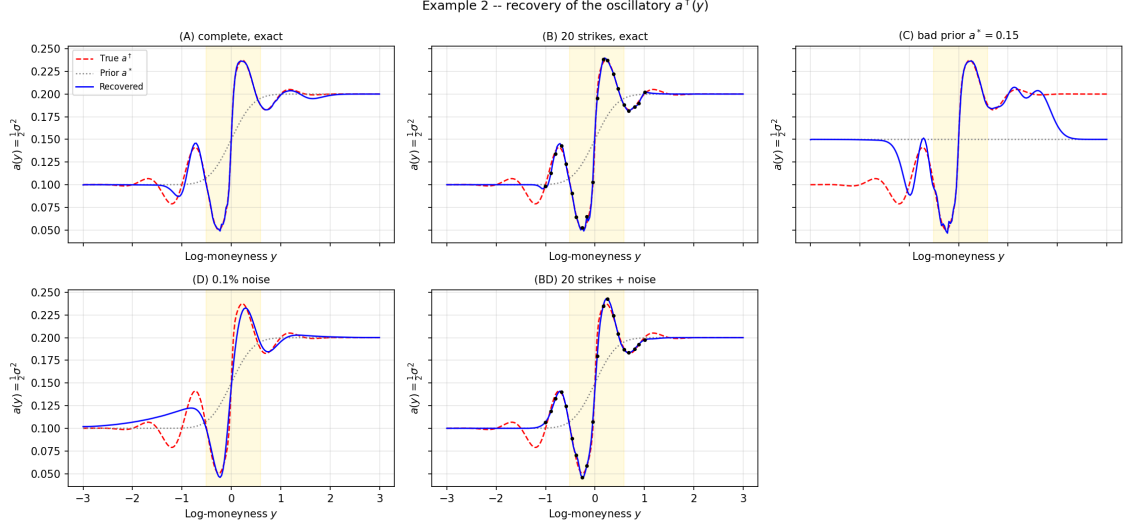
Figure 6: Example 2 of [6]: recovery of the oscillatory local variance a^\dagger(y) (52) (red dashed) for the five test cases. Blue: recovered a(y) ; grey dotted: prior a^* ; black dots (B, BD): observed strikes; shaded band: the strikes K = 600 – 1800 tabulated in the paper.
