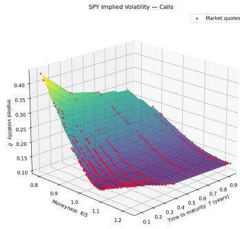
Figure 9: IV surface from all call quotes (including deep ITM, K \ll S ). Deep ITM calls carry noisy implied volatilities due to wide spreads and stale prices.
