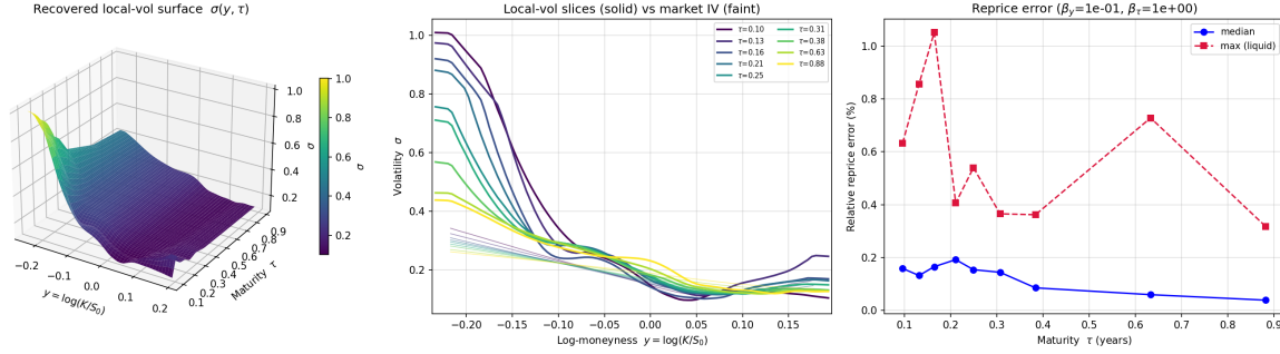
Figure 7.6: Local volatility surface calibrated from SPY quotes on 30 April 2026 ( S_0 = 720.65 , nine maturities), with \beta_y = 0.1 and \beta_\tau = 1 . Left: the recovered surface \sigma(y, \tau) as a 3D mesh. Middle: the recovered local volatility slices (solid) against each maturity's market implied volatility (faint); the local volatility skew is steeper than the implied one. Right: per maturity relative repricing error over liquid strikes (market price at least 0.5% of S_0 ), median and maximum.
