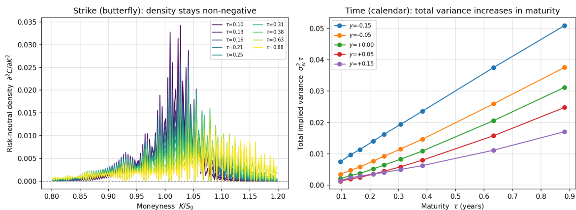
Figure 7.5: No-arbitrage check of the calibrated surface of Figure 7.6. Left: the risk-neutral density \partial_{KK}^2 \mathcal{C} per maturity, non-negative across the observed band (no strike, or butterfly, arbitrage). Right: the total implied variance \sigma_{iv}^2 \tau against maturity at fixed log-moneyness, increasing everywhere (no time, or calendar, arbitrage).
