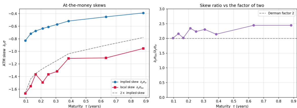
Figure 7.7: The Derman factor of two on the SPY surface of Figure 7.6. Left: the at-the-money implied volatility skew, the recovered local volatility skew, and twice the implied skew. Right: the ratio of local to implied skew against the reference value two. Both skews are read from a quadratic fit in the window |y| \leq 0.05 .
