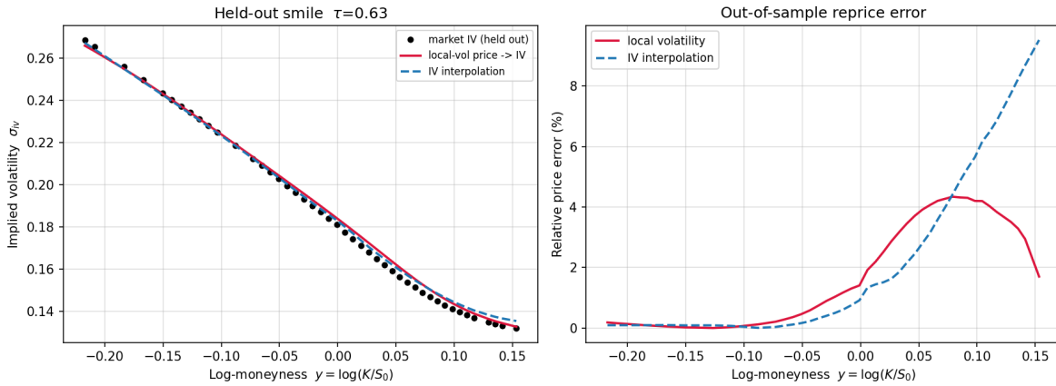
Figure 7.8: Out-of-sample pricing of a held-out expiration (December 2026, \tau = 0.63 ), removed from the calibration and bracketed by \tau = 0.38 and \tau = 0.88 . Left: the held-out market implied volatilities against the local volatility surface price and the implied volatility interpolation, both converted back to implied volatility. Right: relative price error over liquid strikes. The two agree near the money; in the upside wing the local volatility price is the more stable.
