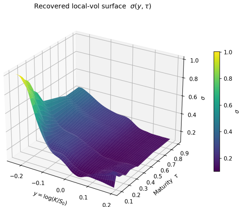
Figure 7.6: Local volatility surface \sigma(y, \tau) calibrated from SPY quotes on 30 April 2026 ( S_0 = 720.65 , eleven maturities), with \beta_y = 0.1 and \beta_\tau = 1 .
