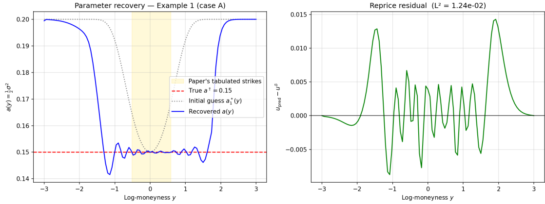
Figure 5: Example 1 (case A) of [6], constant-volatility recovery. Left : recovered a(y) = \frac{1}{2}\sigma^2 (blue) against the true value a^\dagger = 0.15 (red dashed) and the initial guess/prior a_1^* (grey dotted); the shaded band marks the strikes K = 600 – 1800 tabulated in the paper. Right : the repricing residual u_{\text{pred}} - u^\delta at \tau = T .
