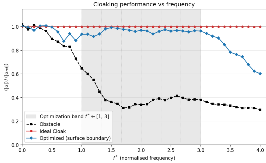
Figure 8: Frequency sweep of the cloak ratio \eta = \langle |\mathbf{u}| \rangle / \langle |\mathbf{u}_{\text{ref}}| \rangle for the broadband 14 \times 10 design trained on the band f^* \in [1, 3] (shaded): the ideal continuous transformation cloak (red, \eta \approx 1 at every frequency), the uncloaked notch (black, dashed), and the broadband optimised cloak (blue). The optimised design holds \eta \approx 0.96 across the entire training band and degrades gracefully outside it.
