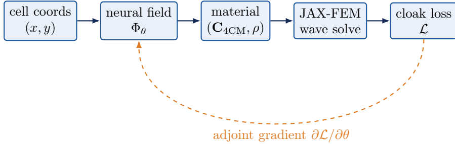
Figure 3: Neural-field design pipeline. Cell-centre coordinates are mapped through a Fourier positional encoding into a four-layer MLP that predicts the four free Cauchy moduli ( C_{11}, C_{12}, C_{22}, C_{66} ) and the density. The piecewise-constant material assignment is expanded to the FEM quadrature points and the cloaking objective is differentiated back through the implicit JAX-FEM adjoint into the network weights.
