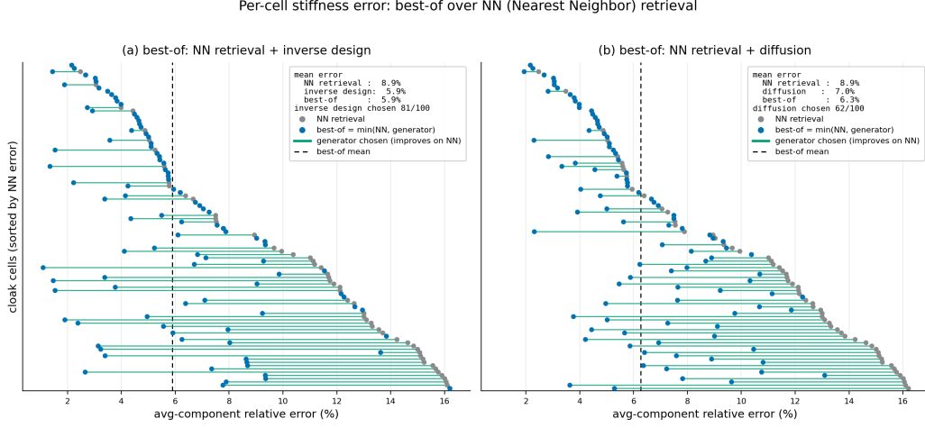
Figure 10: Per-cell stiffness-matching error over the 100 cloak cells for the two realisation methods against NN (Nearest Neighbor) retrieval: (a) NN + inverse design, (b) NN + diffusion. Each row is a cell; the bar links the NN error (grey) to the per-cell best-of selection (blue, the lower-error of the two). Best-of lowers the mean avg-component stiffness error from 8.9% to 5.9% (inverse) and 6.3% (diffusion); cells are sorted by NN error.
