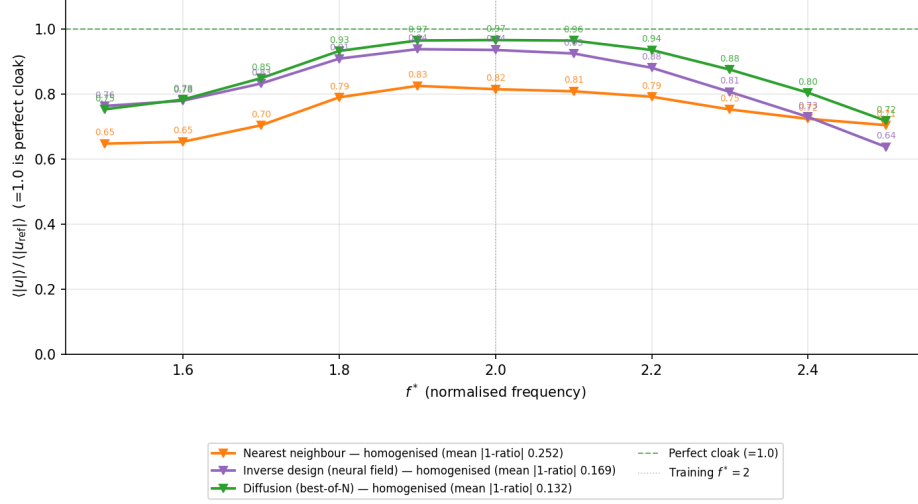
Figure 10: Frequency sweep of the cloak ratio \eta(f) = \langle |u| \rangle / \langle |u_{\text{ref}}| \rangle for the three microstructure-realisation methods on the matched homogenised 20 \times 15 cloak: nearest-neighbour dataset snap (orange), neural-field inverse design (purple), and best-of- N diffusion (green). Diffusion stays closest to the perfect-cloak line ( \eta = 1 ) across the band and has the smallest mean distortion; the dashed line is the training frequency f^* = 2 .
