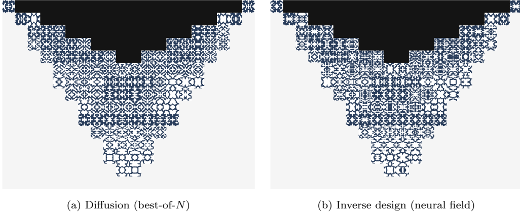
Figure 11: Explicit realisation of the triangular carpet cloak from a single cement phase: the 100 generated 50 \times 50 unit cells tiled at the macro-cell positions they occupy in the cloak. Cement is dark, void white; the black inverted triangle is the surface notch and the light grey region is the surrounding half-space. (a) Best-of- N diffusion and (b) neural-field inverse design produce visibly different but equally manufacturable patterns for the same optimised per-cell targets.
