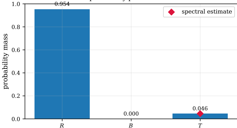
Late-time probability partition in barrier test
