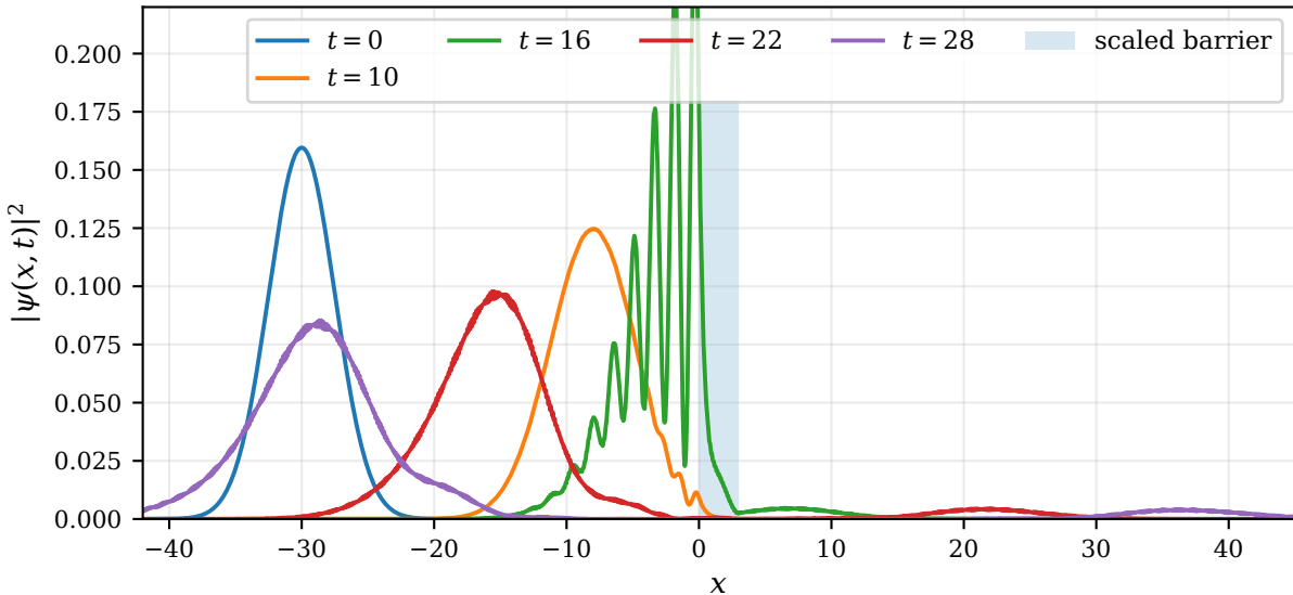
Finite barrier scattering: incident, reflected, and transmitted packets
