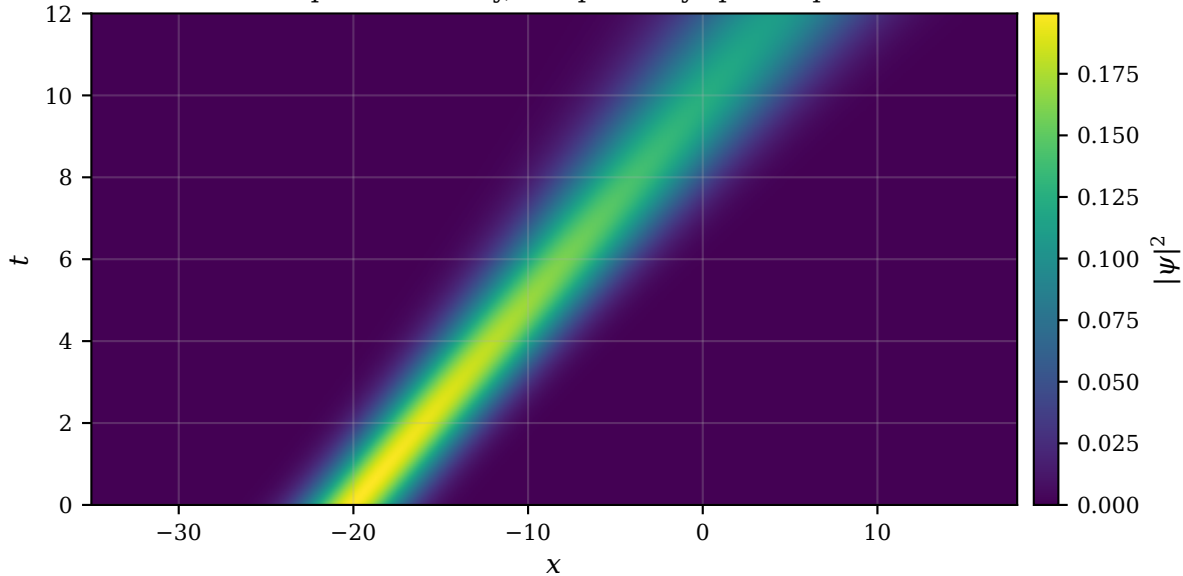
Free wavepacket density, computed by split-step Fourier
