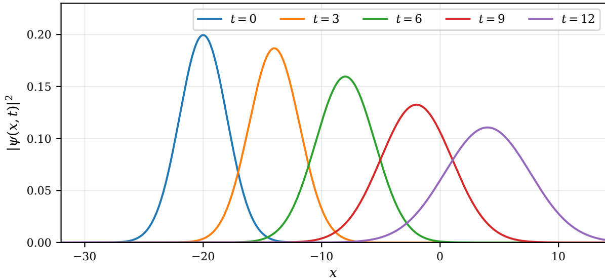
Free Gaussian wavepacket: translation and dispersion
