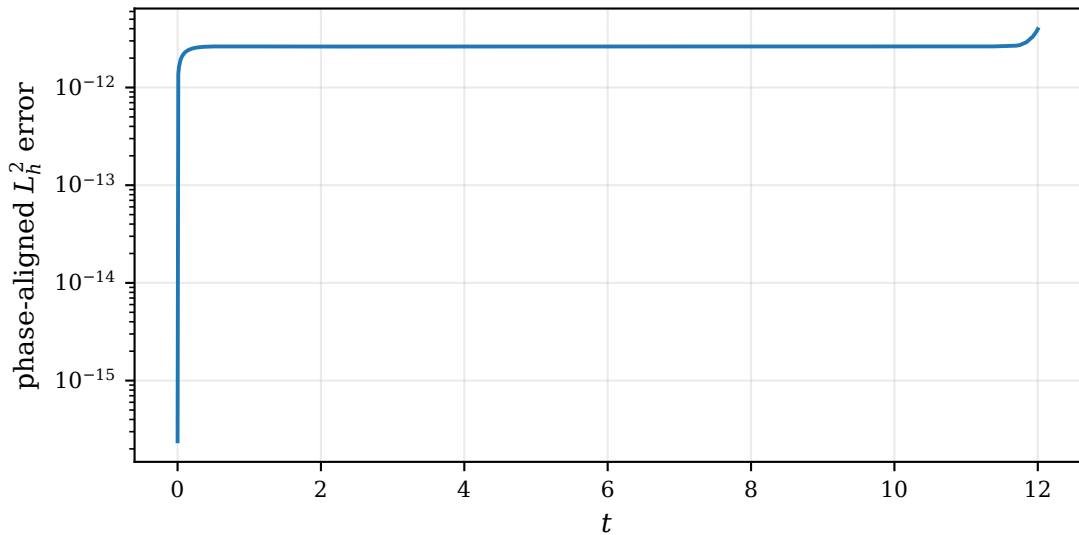
Full-state analytic validation for free propagation
