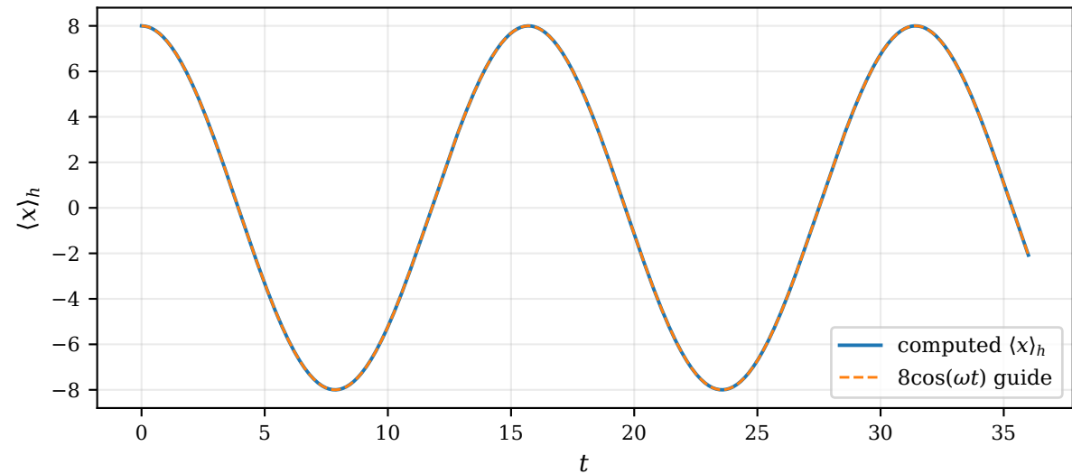
Harmonic oscillator center-of-mass diagnostic
