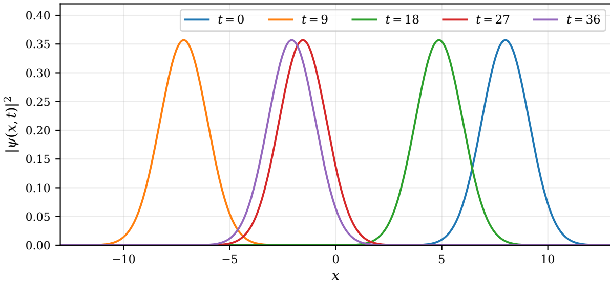
Harmonic oscillator: oscillation of a localized packet
