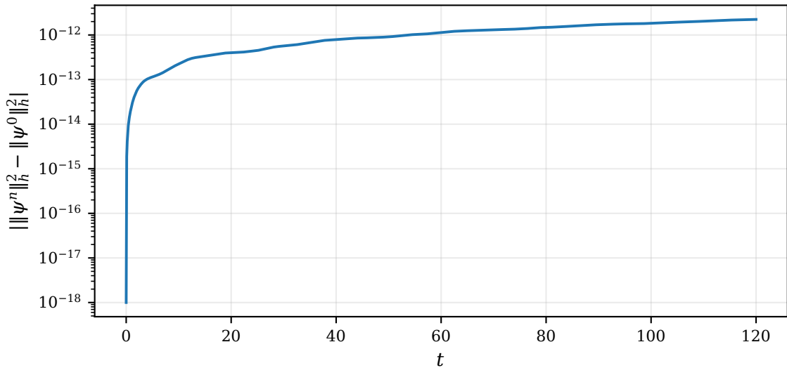
Long-time norm preservation diagnostic
