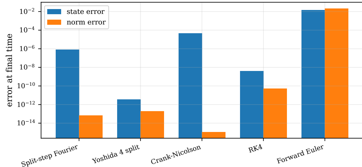
Finite-dimensional method comparison
