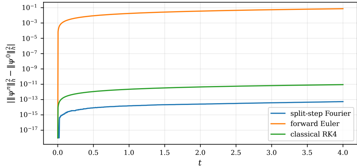
Norm error for unitary and non-unitary time steppers
