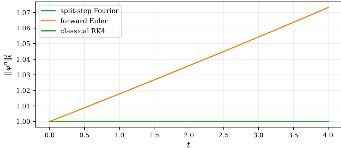
Discrete norm squared over time
