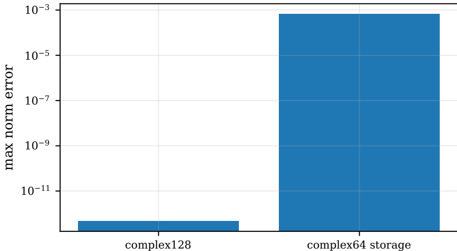
Precision sensitivity for stored split-step states
