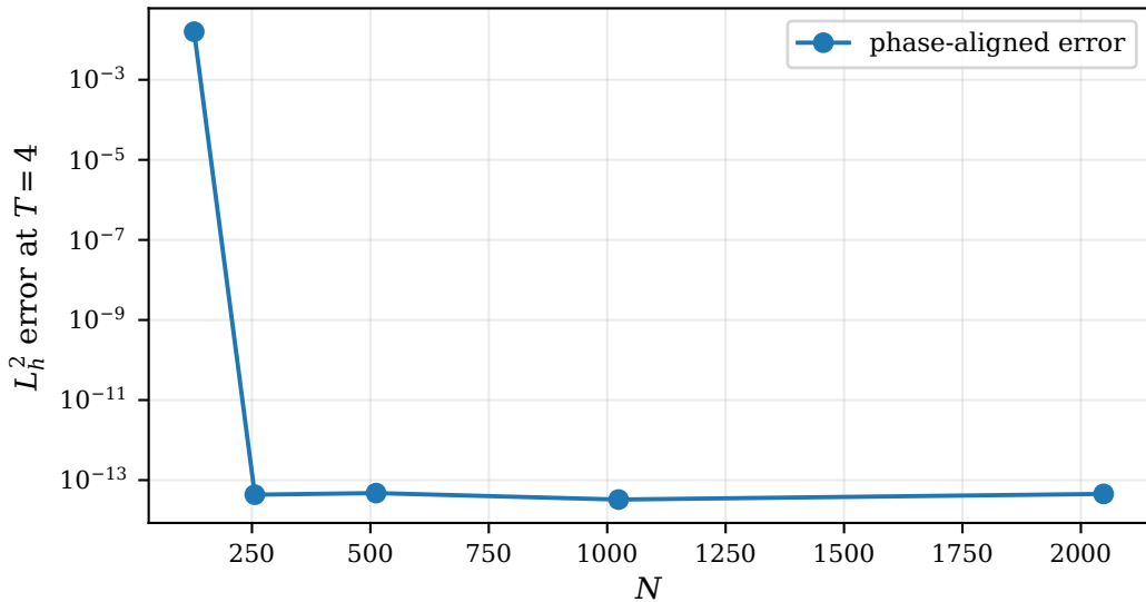
Spatial refinement diagnostic for a free Gaussian packet
