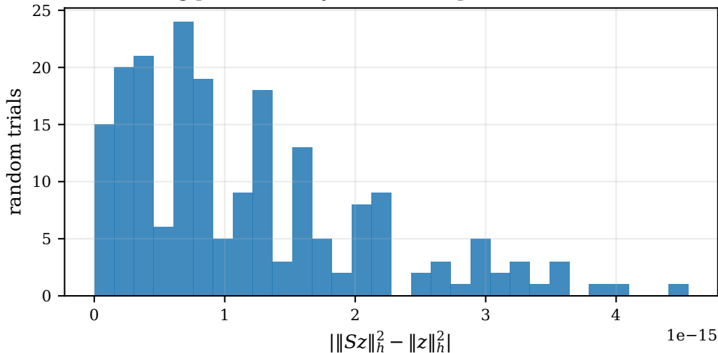
Floating-point unitarity defect for explicit small-matrix test
