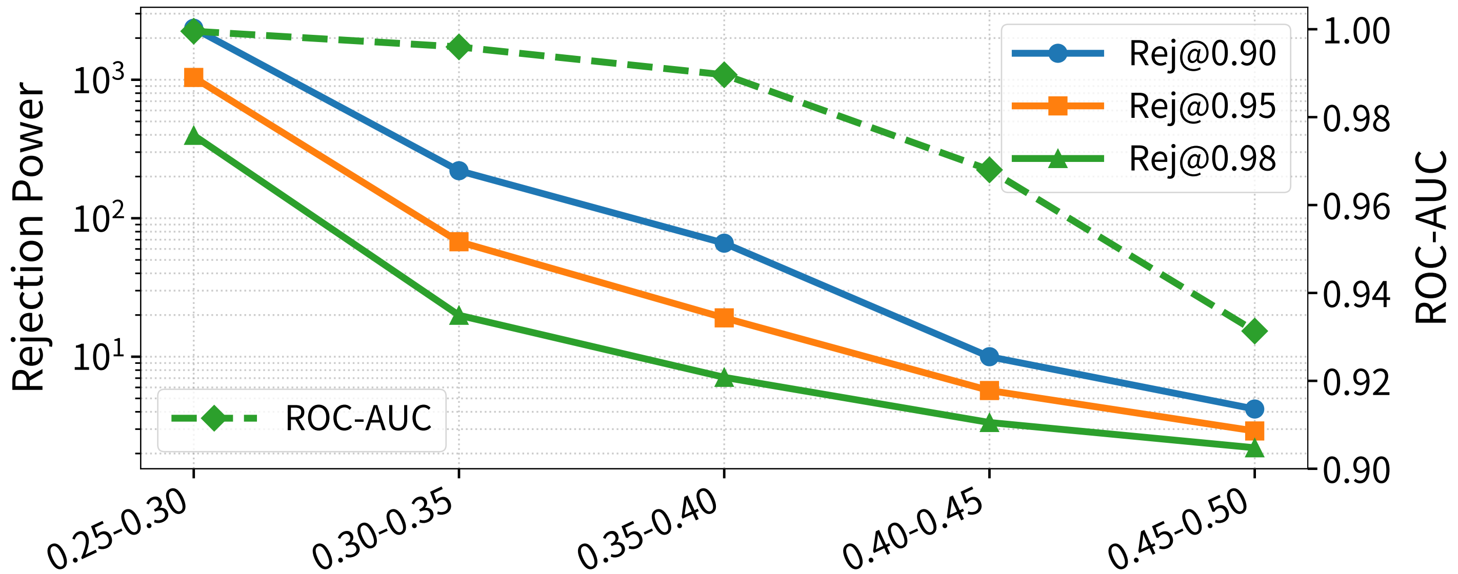
Performance by beta range
