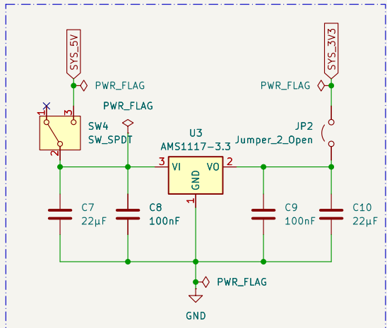
3V3 Regulator
