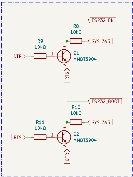
Auto-Download Circuit
