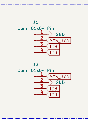
I2C Pins
