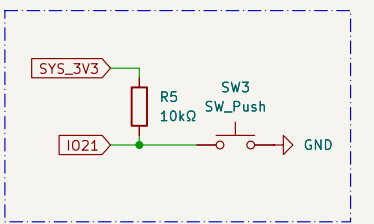
User's Button
