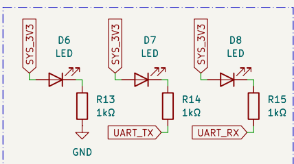
LED Indicators
