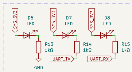
LED Indicators
