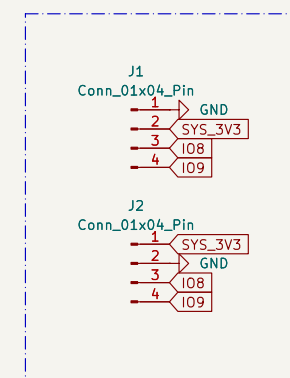
I2C Pins
