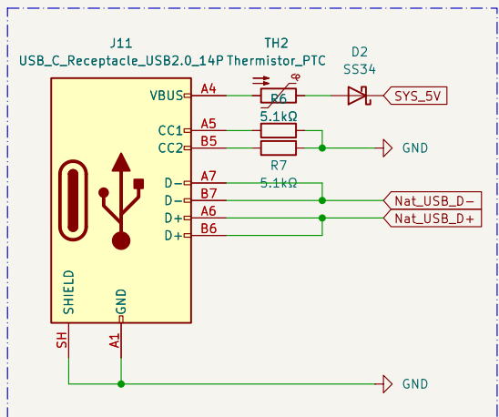
Native USB
