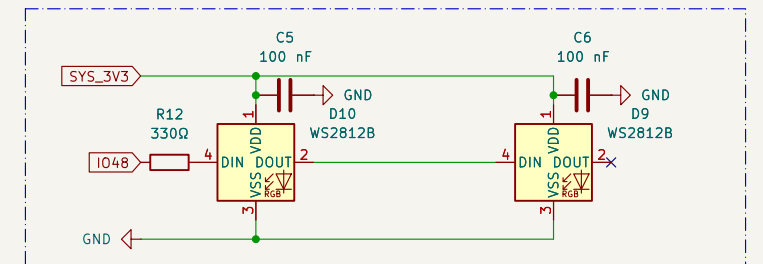
Addressable RGB Status LEDs
