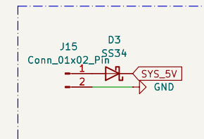
V_in Pins
