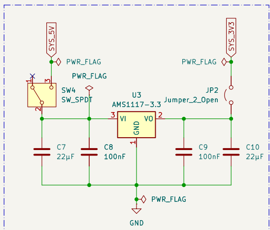
3V3 Regulator
