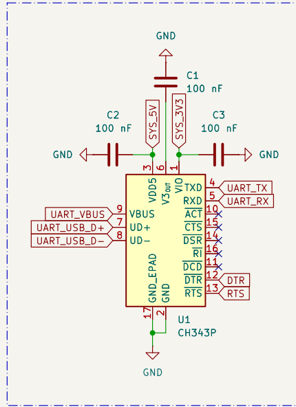
UART Bridge
