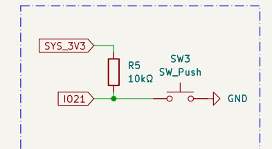
User's Button
