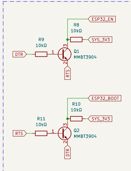
Auto-Download Circuit
