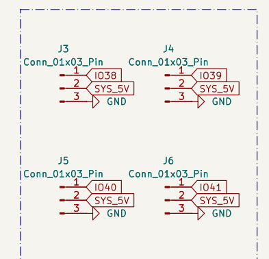
Servo Motor Pins
