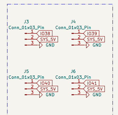
Servo Motor Pins
