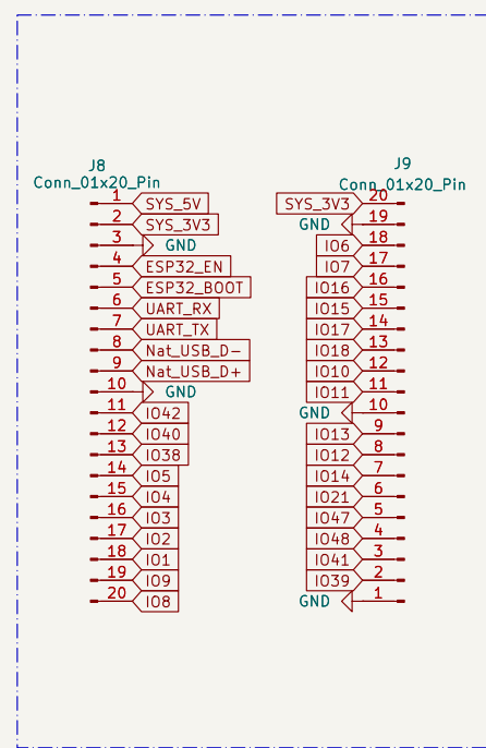
Breakout Pins
