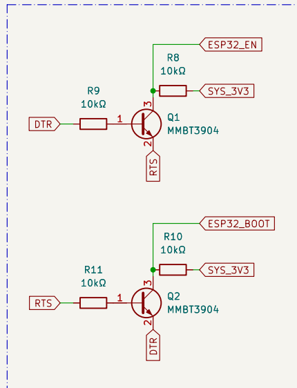
Auto-Download Circuit
