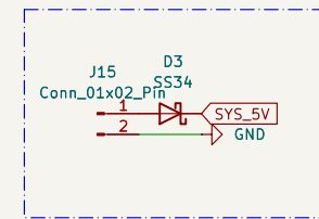
V_in Pins
