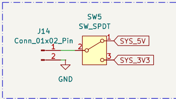
V_out Pins
