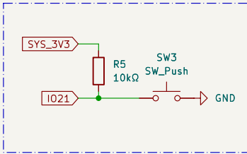
User's Button
