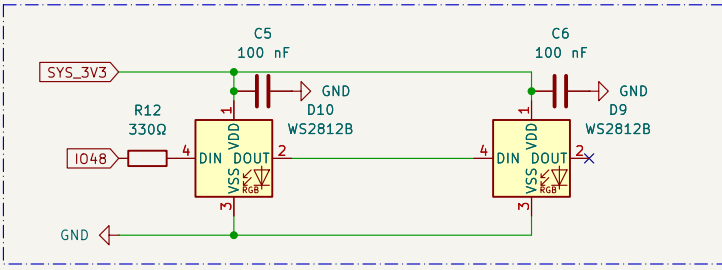
Addressable RGB Status LEDs
