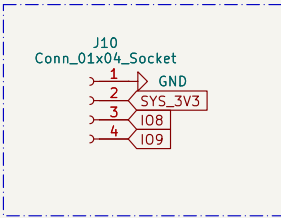
I2C Connector
