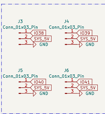
Servo Motor Pins
