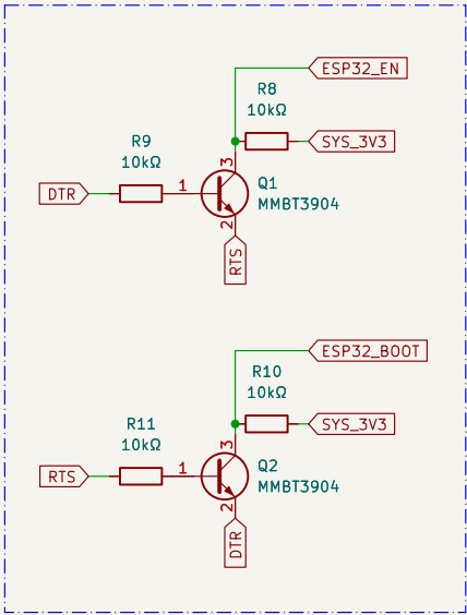
Auto-Download Circuit
