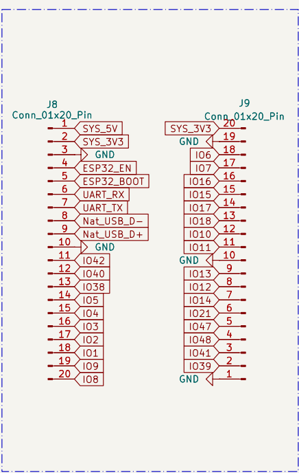
Breakout Pins
