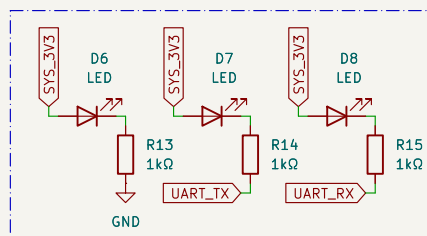
LED_Indicators
