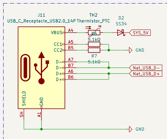
Native USB
