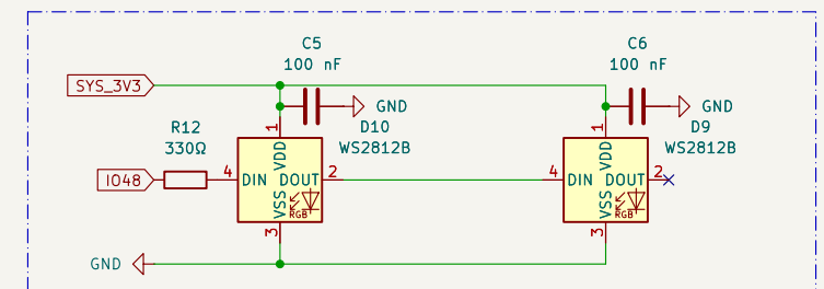
Addressable RGB Status LEDs
