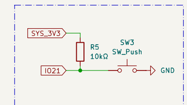
User's Button
