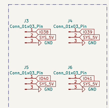
Servo Motor Pins
