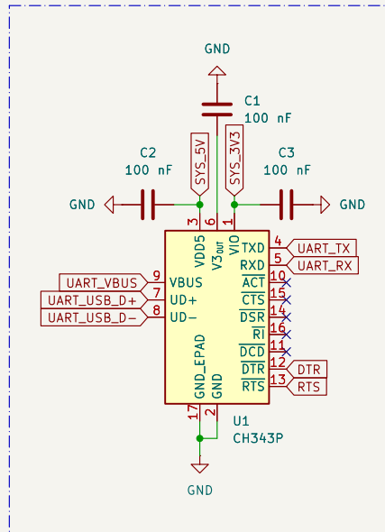
UART Bridge
