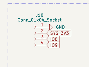
I2C Connector
