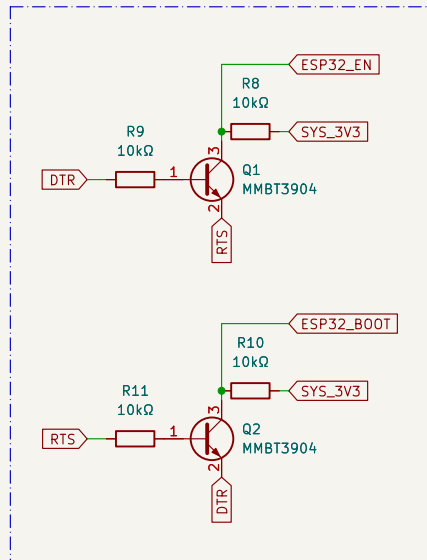
Auto-Download Circuit
