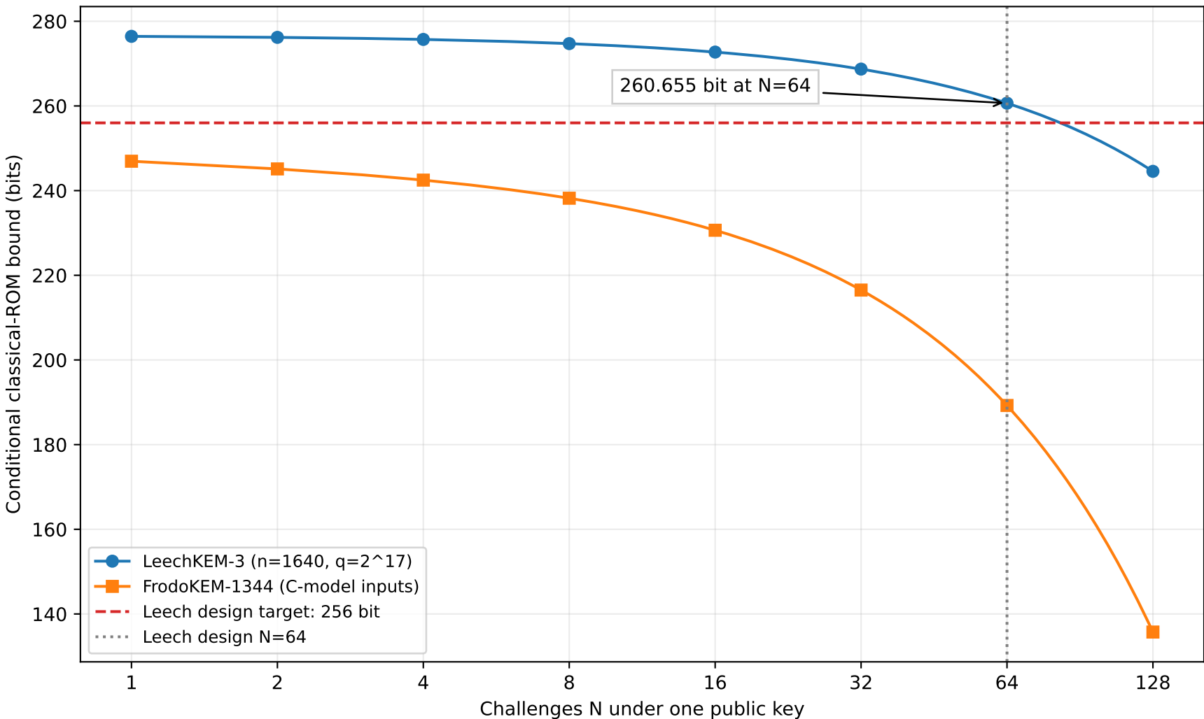
Core-SVP/C-LSF: normalized IND-CCA reduction estimates
