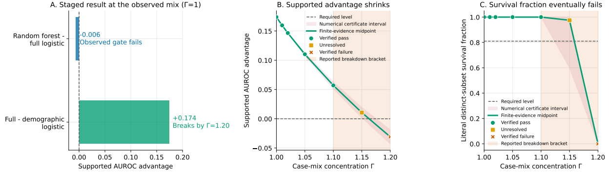
Figure 7: Observed-anchored AUROC case-mix breakdown in the Bank Marketing temporal evaluation. Panel A applies the observed gate before the computational challenge. Panels B and C show the supported-magnitude and literal-survival profiles for the positive control under increasing within-class concentration. The ribbon is the numerical certificate interval; markers distinguish verified passes, unresolved values, and verified failures. The shaded region is the reported breakdown bracket. This is the M = 1 , K_E = 1 , K_C = 2 , J = 80 projected boundary of the full construction.
