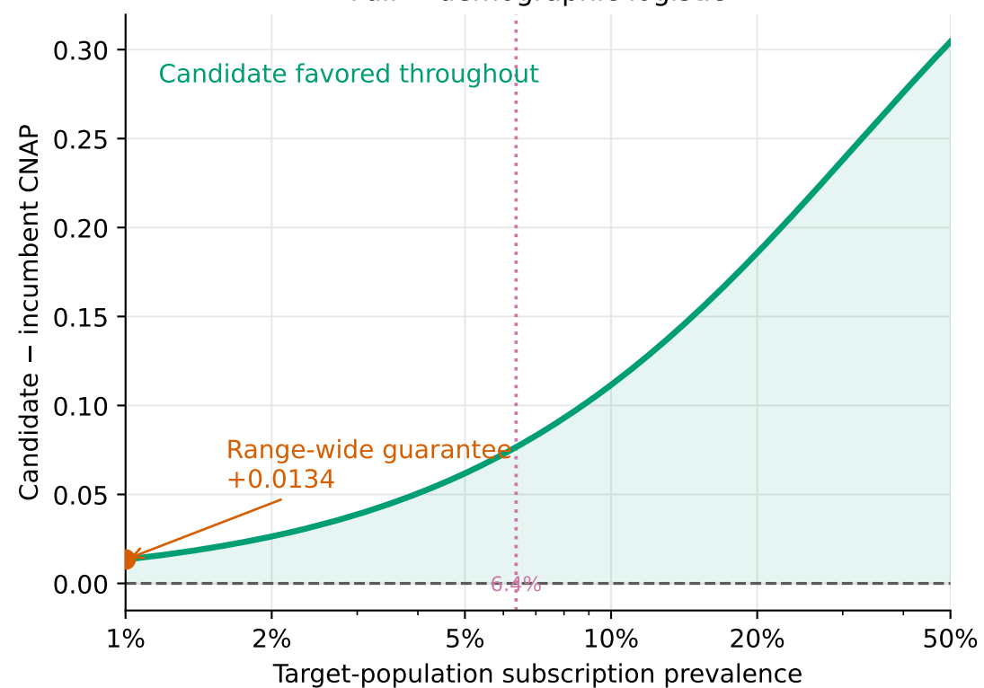
B. Positive control Full – demographic logistic
