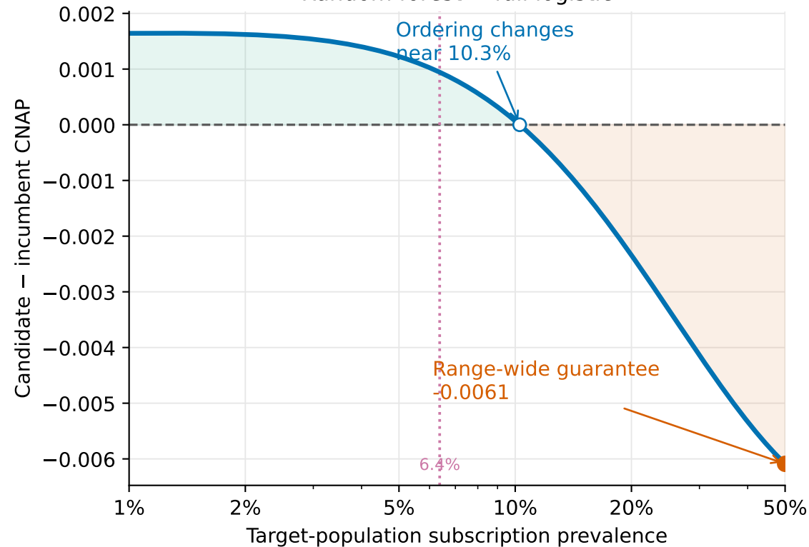
A. Close comparison Random forest – full logistic
