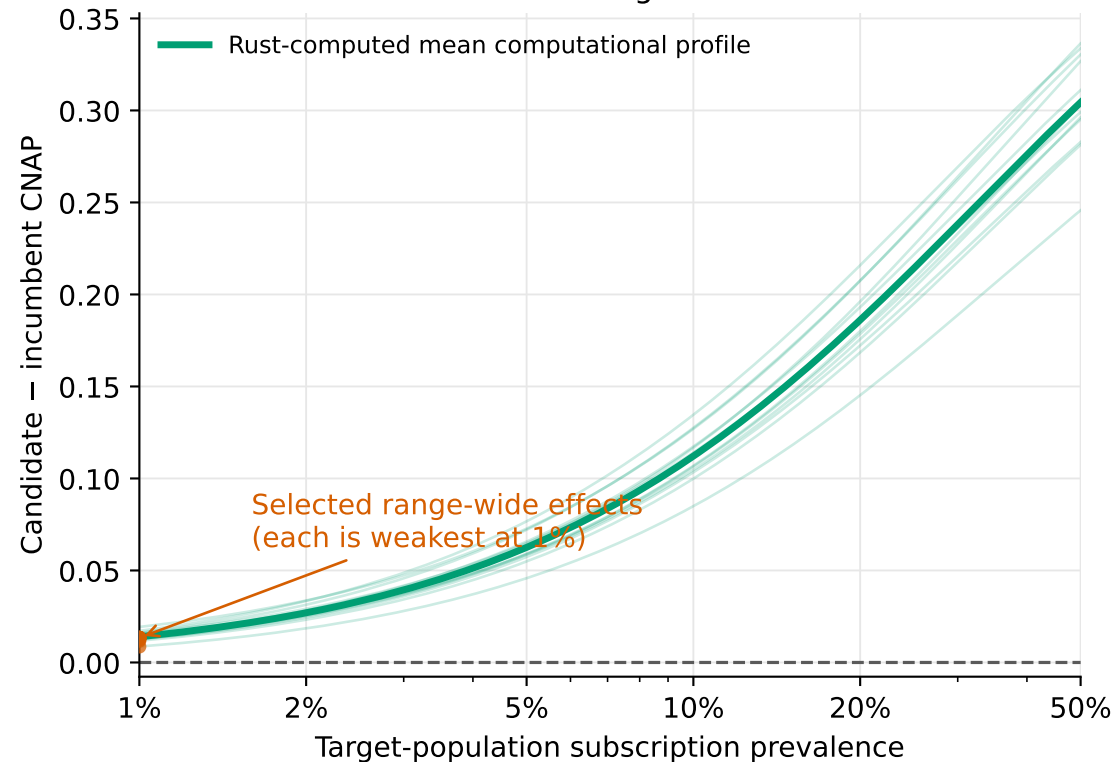
A. Each complete replication faces the full range Dots mark its range-wide result
