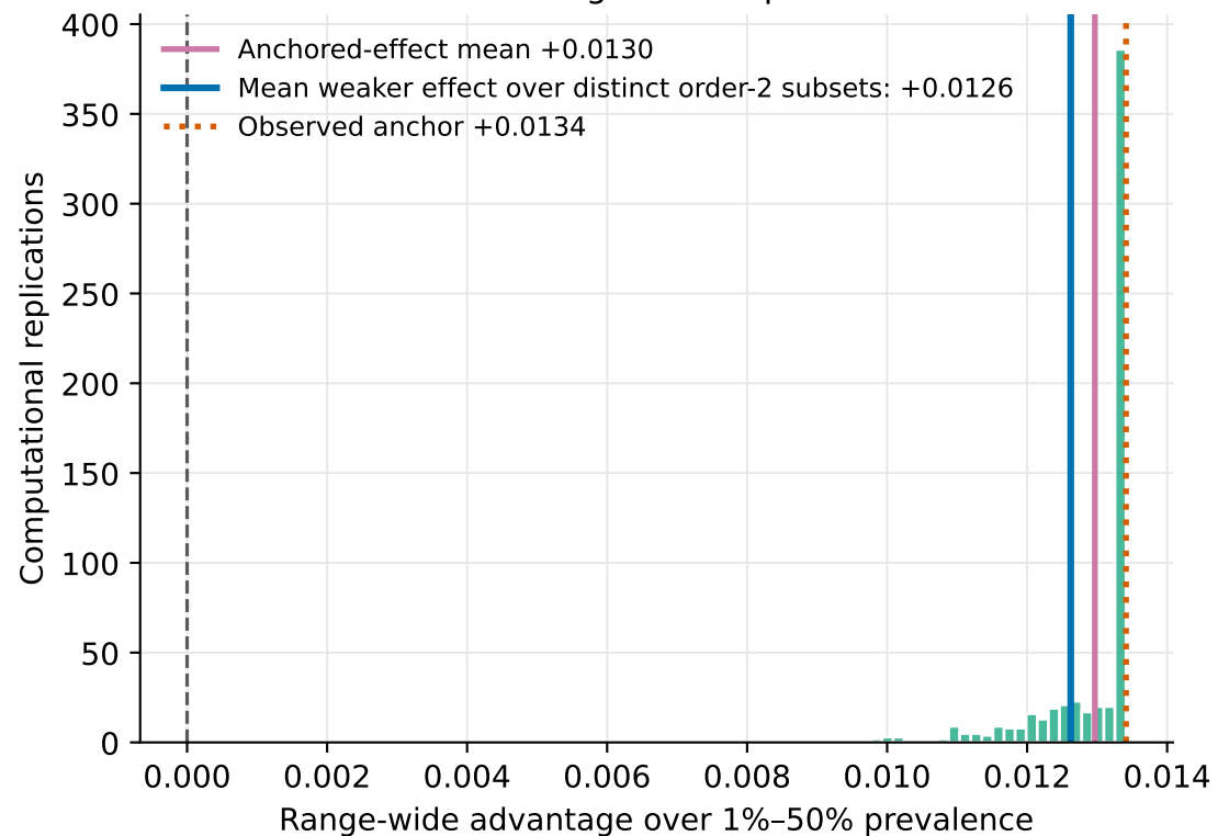
B. Finite list of range-wide replication effects
