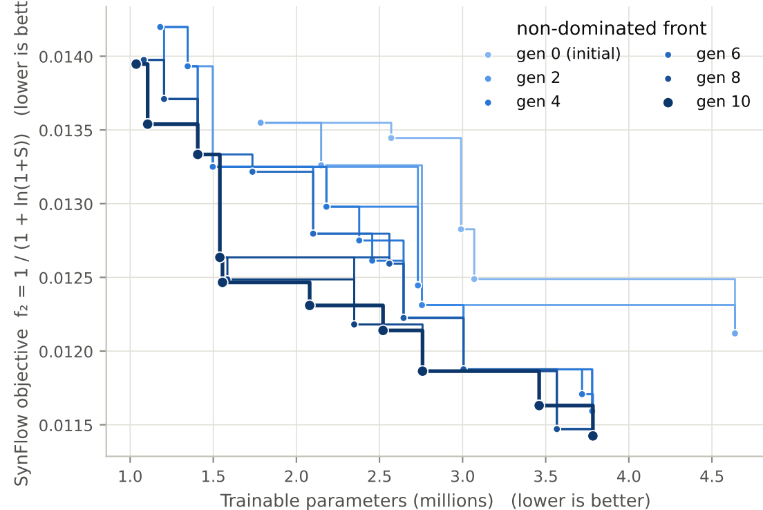
Pareto-front evolution across generations
