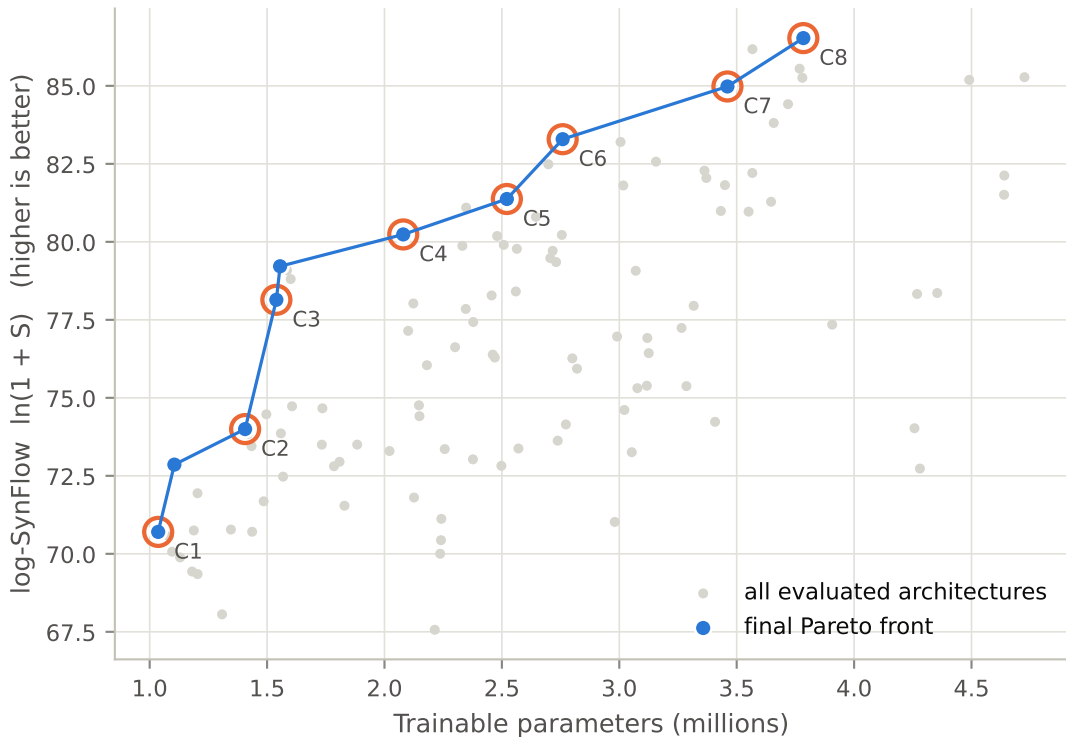
Final Pareto front on the log-SynFlow scale
