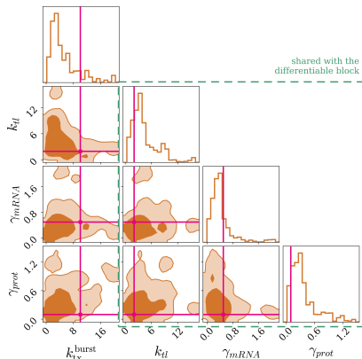
■ Regulator · ABC-SMC all 6 parameters jointly, 4 shown
