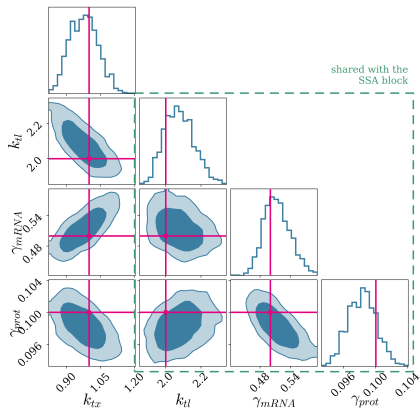
■ Differentiable block · NUTS all 8 parameters jointly, 4 shown
