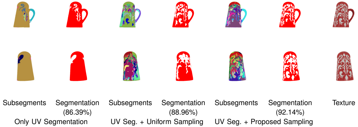
FIGURE 12. Ablation Study of Camera Sampling Strategies. We compare subsegment quality and segmentation results under three settings: (1) UV-only segmentation, (2) UV segmentation with uniform camera sampling, and (3) UV segmentation with our proposed visibility-aware camera sampling. Incorporating multiple 3D camera views significantly improves subsegment detail, and our visibility-aware sampling yields more coherent texture mappings than uniform sampling. We also report segmentation accuracy, defined as the proportion of correctly classified pixels within the visible area.
