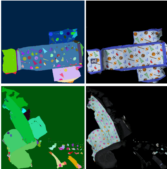
FIGURE 13. UV-texture segmentation results by SAM-HQ [3]: We observe inconsistent segmentation of fine texture details.
