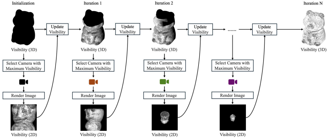
FIGURE 6. Camera sampling. We greedily select a set of cameras that maximizes the visibility of 3D surfaces.
