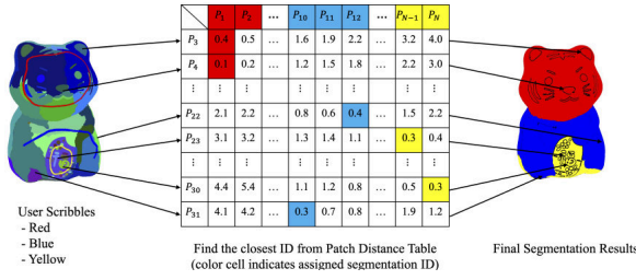
FIGURE 7. Propagation of Subsegment IDs. Based on the user scribbles, we assign the segmentation ID to the non-scribbled subsegments by checking the closest user scribble in the subsegment distance table. This yields the final segmentation results.
