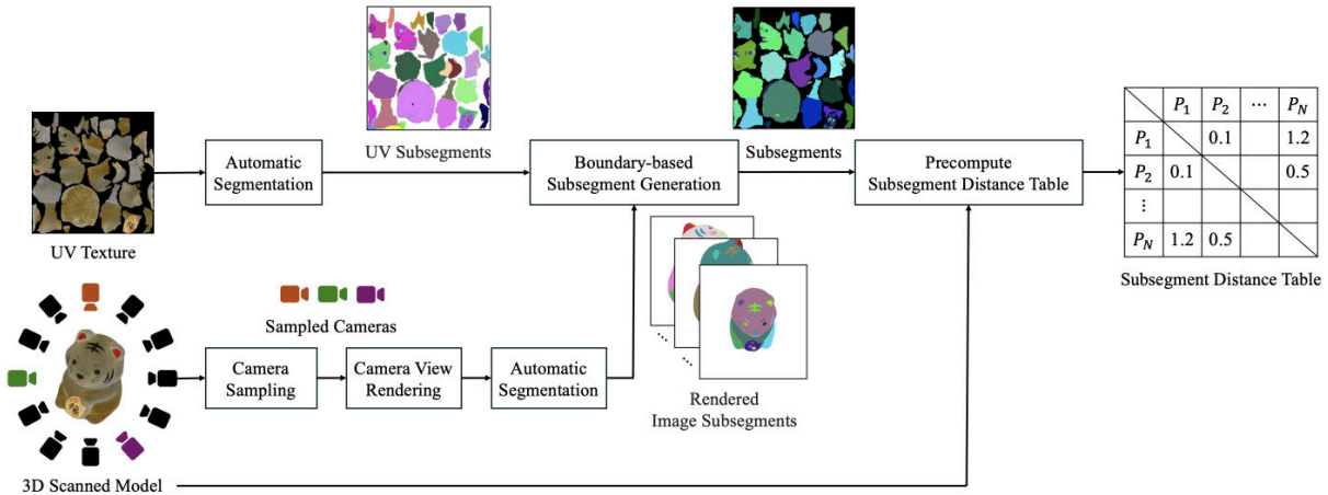
FIGURE 5. Overview of preprocessing. The system first generates two kinds of subsegments, UV subsegments and rendered image subsegments. Then, these two subsegments are merged in boundary-based subsegment generation step. Finally, the system precomputes distances between subsegments to generate a subsegment distance table.
