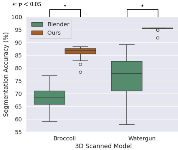
FIGURE 10. The boxplot results illustrate that our approach enhances segmentation accuracy in nearly every instance.
