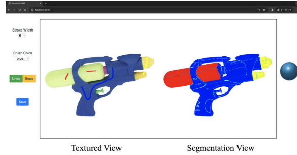
FIGURE 2. Screenshot of our system. It consists of brush adjustment (brush size, color), undo/redo operation, save operation of UV map, and camera control. On the main screen, the user can simultaneously check both textured mesh and segmentation mesh which always visualize the boundaries by light blue color. Once the scribble is added to a textured view, the segmentation results are updated. In the Figure's example, the user added three scribbles (red, blue, yellow), from which the segmentation is automatically estimated.
