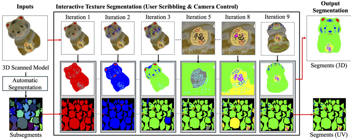
FIGURE 4. Workflow of our interactive texture segmentation using a 3D scanned model. Automatic segmentation divides the texture into small subsegments in a pre-processing step. The user then iteratively classifies the subsegments into segments by drawing scribbles on the 3D model. The segment ID of a subsegment is set to the ID of the nearest stroke.
