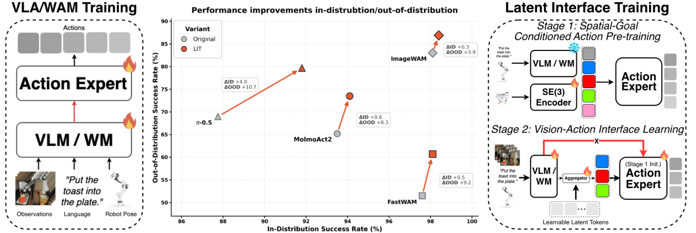
Fig. 1. Training paradigms and generalization performance. Standard training conditions the action expert on visual representations (left). LIT (right) first learns a spatial-goal-conditioned action prior without images to avoid relying on visual correlations during pre-training (Stage 1), then introduces visual conditioning through a pose-supervised latent interface (Stage 2). Across four VLA and WAM architectures, LIT improves out-of-distribution success rates while preserving or improving in-distribution success rates (center).
