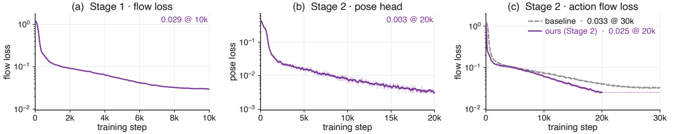
Fig. 7. Training dynamics on MolmoAct2. (a) Stage 1 action flow-matching loss. (b) Stage 2 pose-reconstruction loss. (c) Action flow-matching loss during visual policy training. LIT uses 10K Stage 1 and 20K Stage 2 steps, matching the baseline’s 30K-step total budget. LIT’s Stage 2 action loss reaches a lower value than the baseline’s final loss. Panel (c) counts visual training steps; the 0.63\times ratio compares losses at 20K steps.
