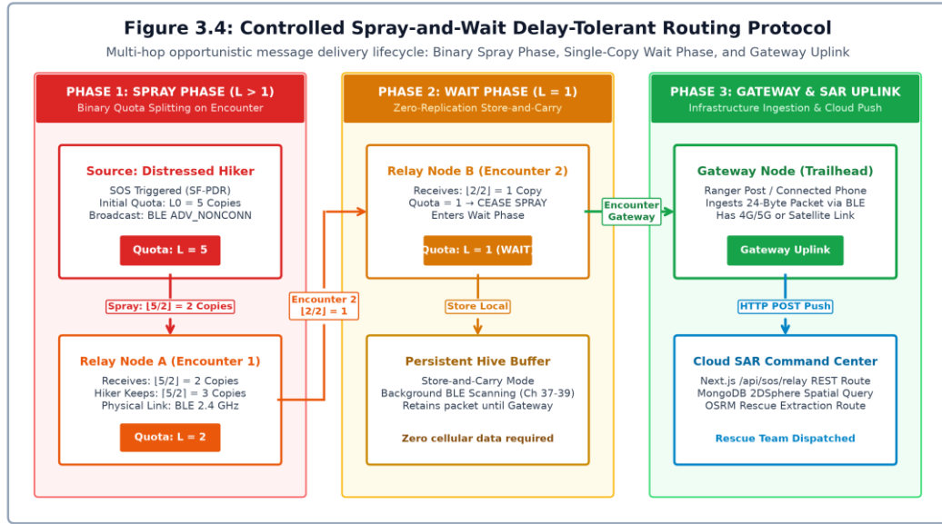
Figure 3.4: Controlled Spray-and-Wait Delay-Tolerant Routing Protocol
