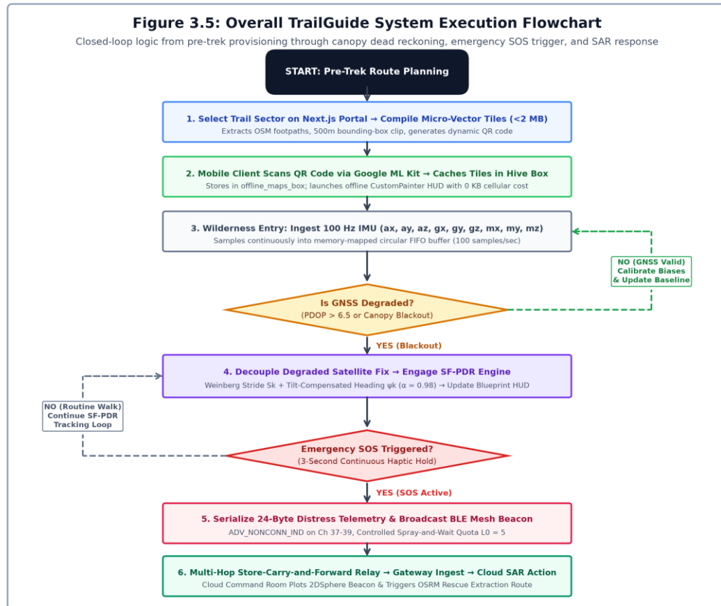
Figure 3.5: Overall TrailGuide System Execution Flowchart
