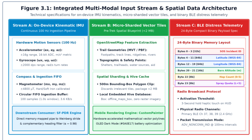
Figure 3.1: Integrated Multi-Modal Input Stream & Spatial Data Architecture
