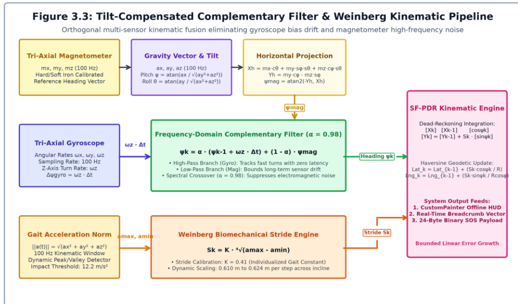
Figure 3.3: Tilt-Compensated Complementary Filter & Weinberg Kinematic Pipeline
