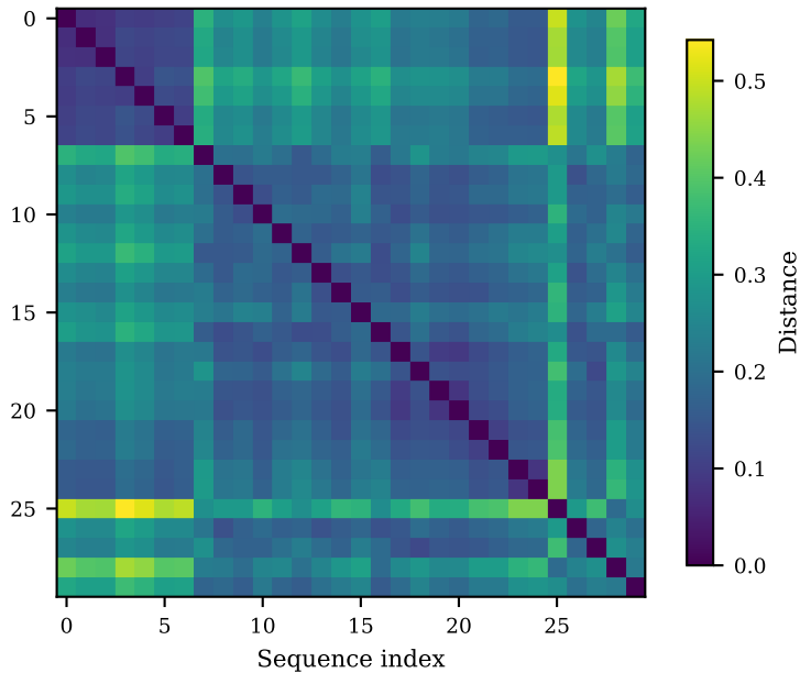
L_1 ( k -mer composition) distance D_c
