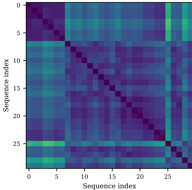
p -adic distance D_p
