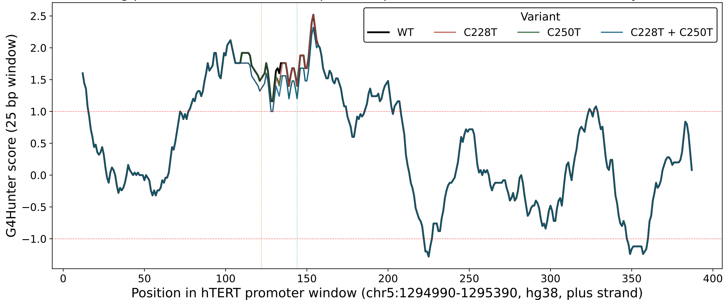
G4-forming potential across the hTERT proximal promoter with C228T / C250T overlays
