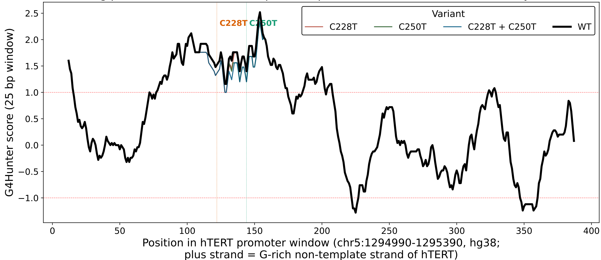
G4-forming potential across the hTERT proximal promoter with C228T / C250T overlays
