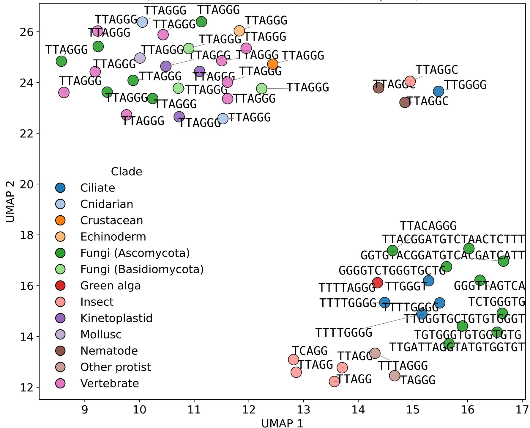
Telomeric tandem-repeat embeddings across eukaryotes (Nucleotide Transformer v2, 500M, multi-species)
