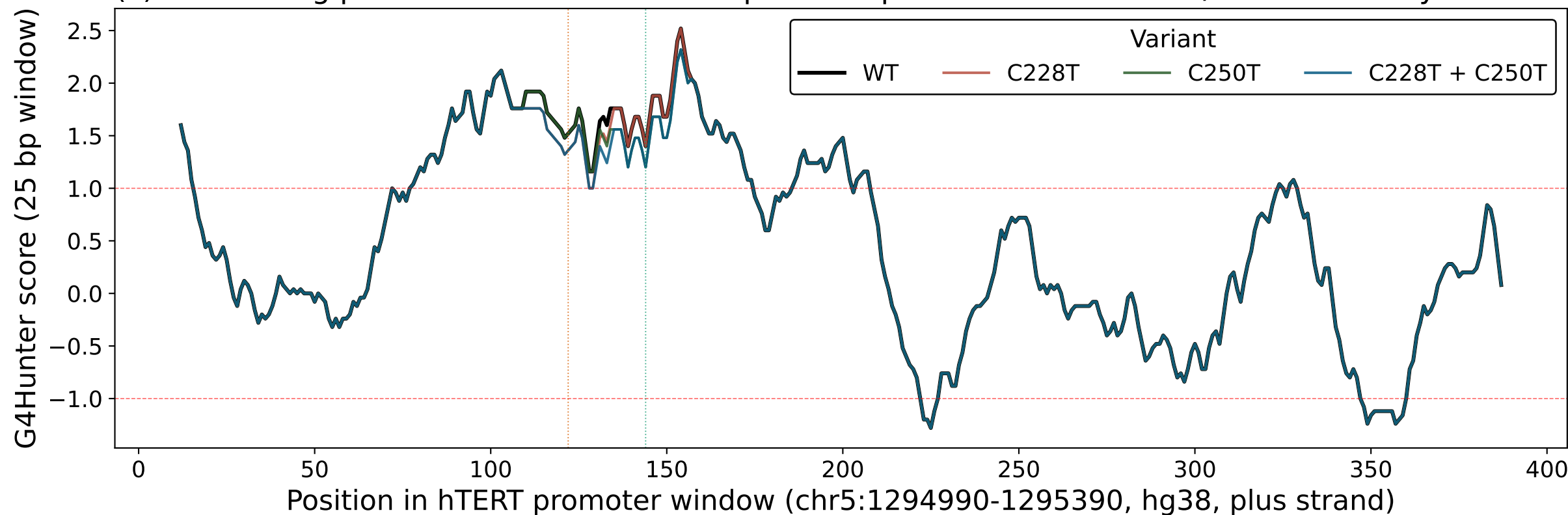
(ii) G4-forming potential across the hTERT proximal promoter with C228T / C250T overlays
