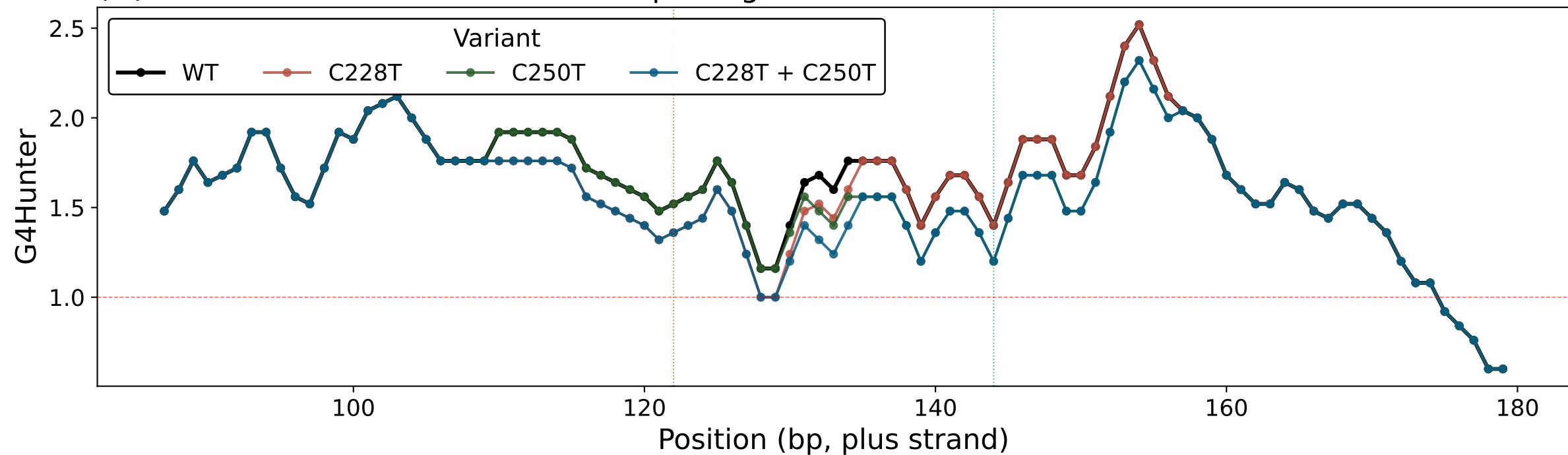
(iii) Zoom on the C228T / C250T hotspot region
