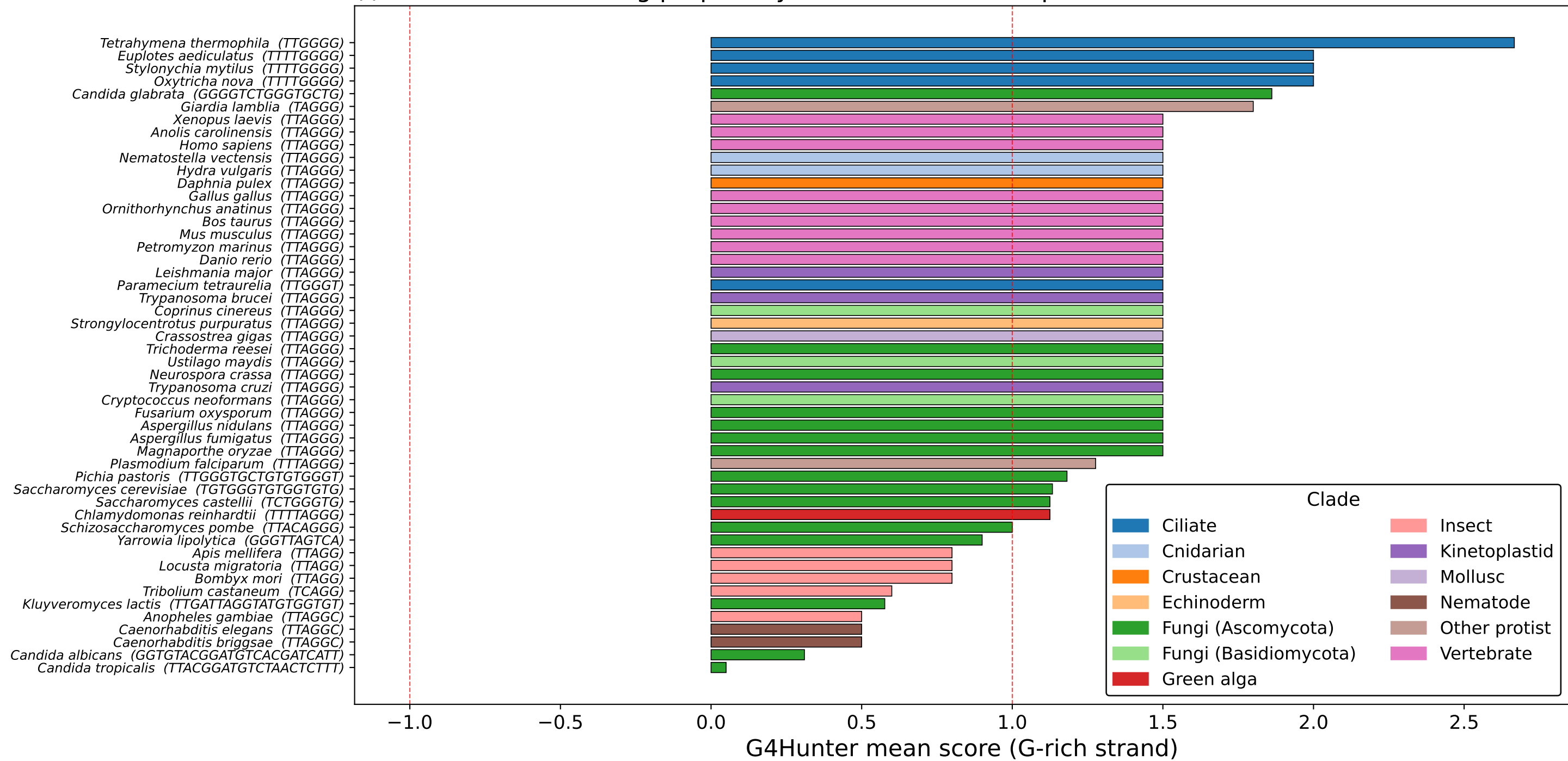
(i) Predicted G4-forming propensity of tiled telomeric repeats
