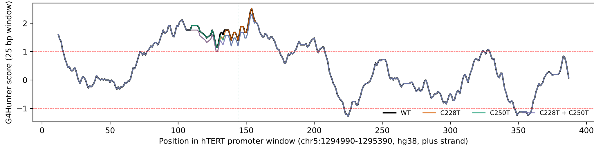
(ii) G4-forming potential across the hTERT proximal promoter with C228T / C250T overlays
