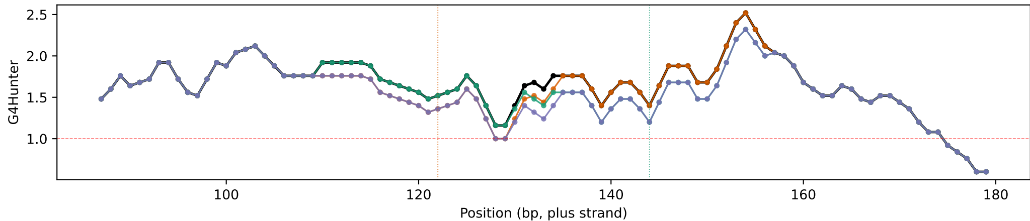
(iii) Zoom on the C228T / C250T hotspot region
