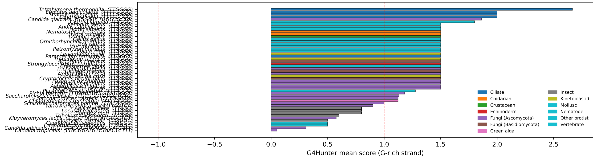
(i) Predicted G4-forming propensity of tiled telomeric repeats
