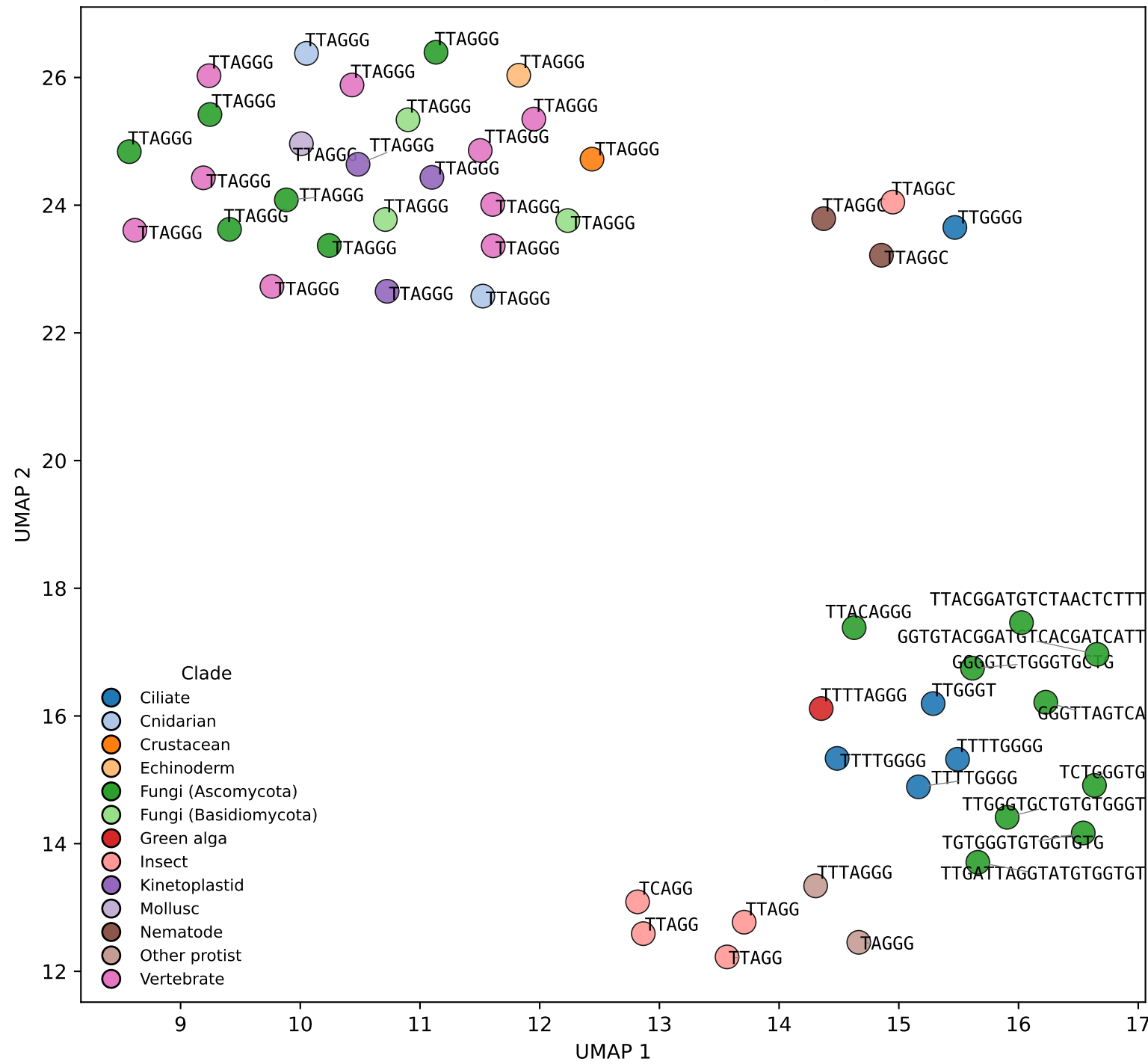
Telomeric tandem-repeat embeddings across eukaryotes (Nucleotide Transformer v2, 500M, multi-species)
