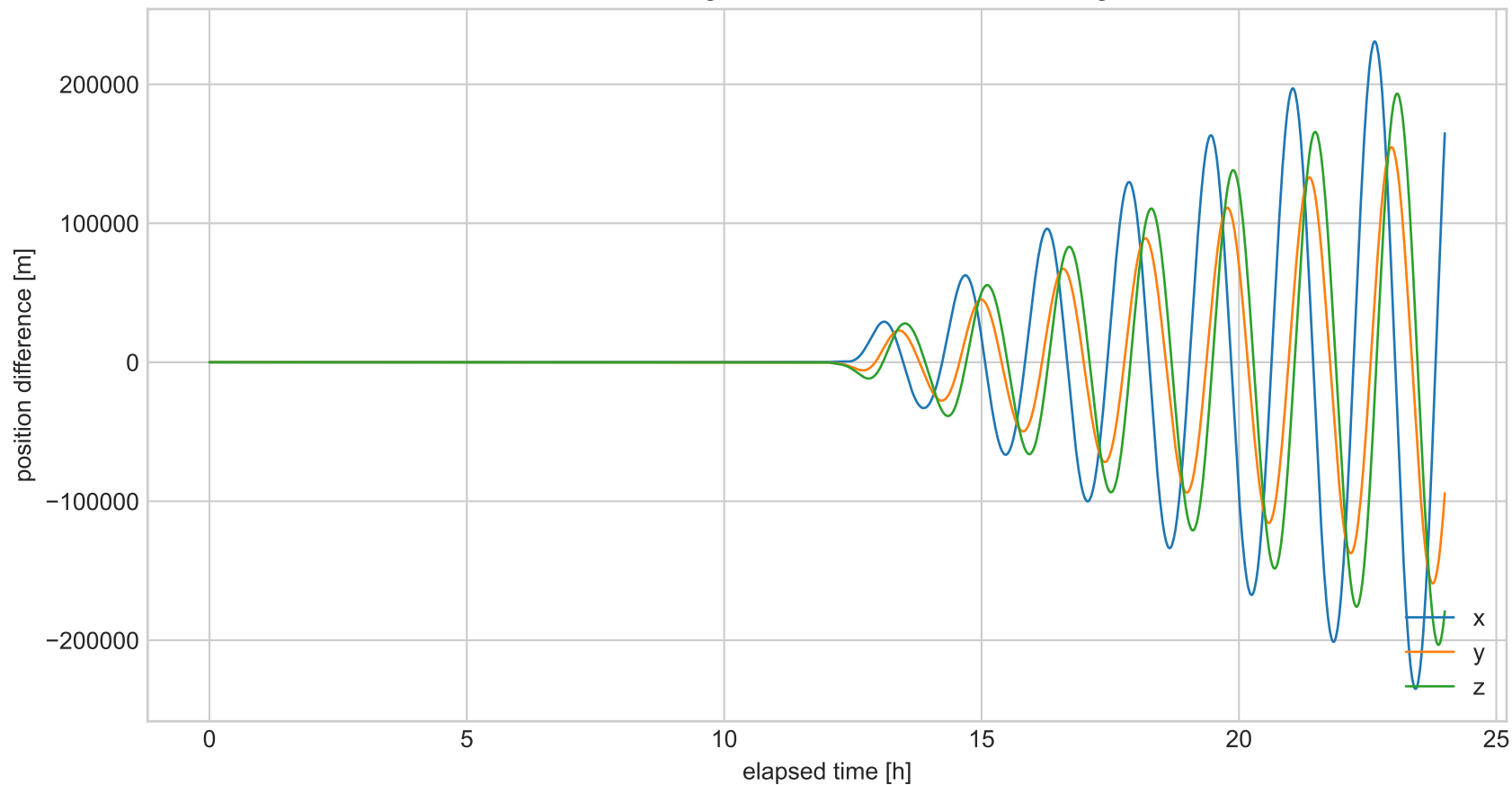
Position difference: numerical-ground-track.csv vs numerical-ground-trackJ2.csv
