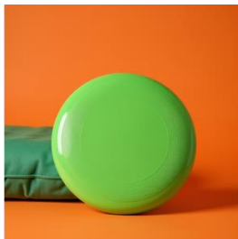
Flux.1-Dev
